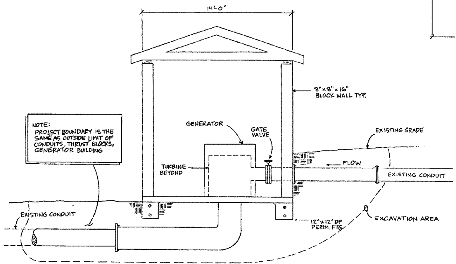
Section View - Powerhouse scale 1" = 30 ft.
