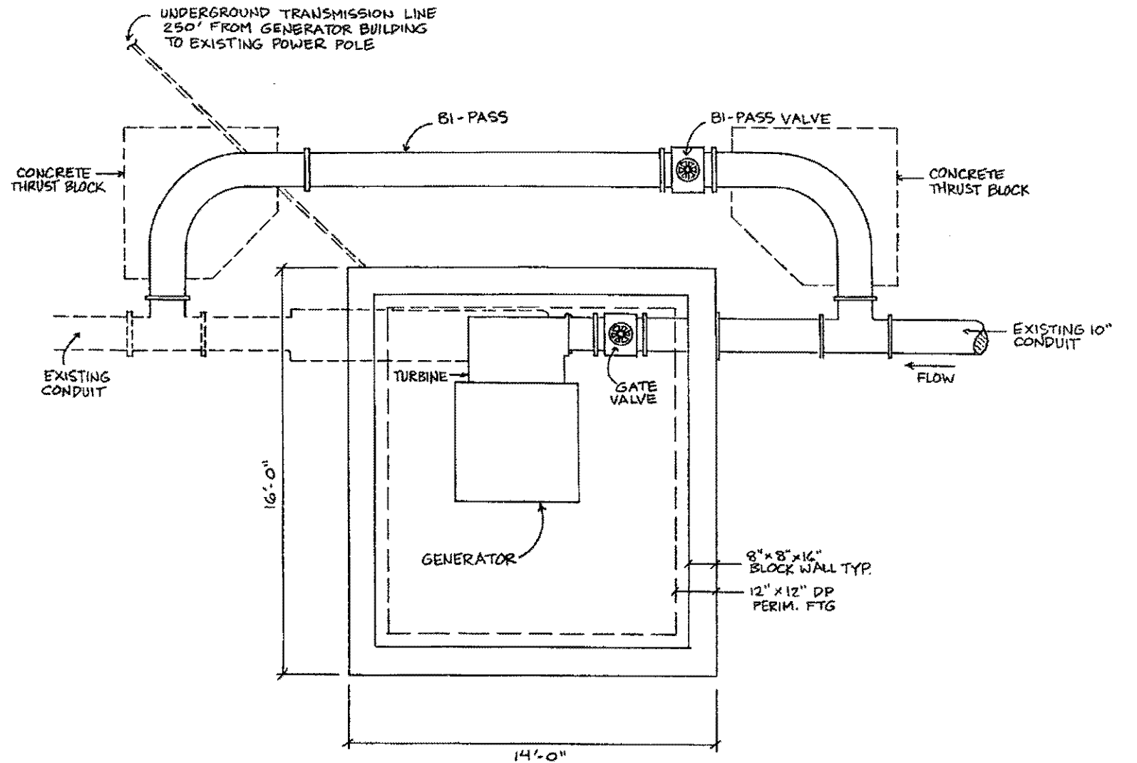
Plan View - Powerhouse scale 1" = 30 ft.
