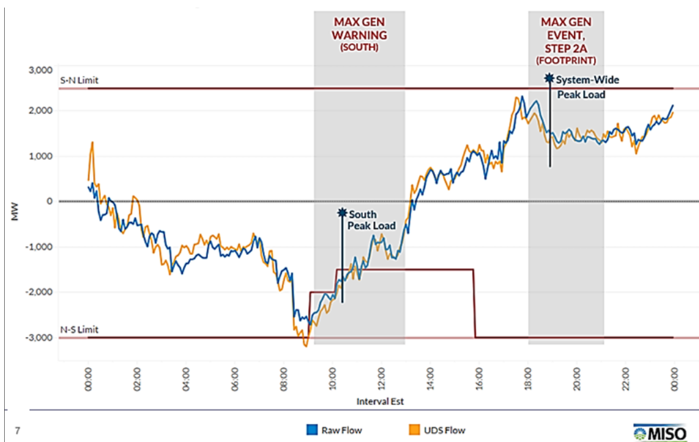
Figure 42: MISO Regional Directional Transfer (RDT) Flow, 156 December 23, 2022
